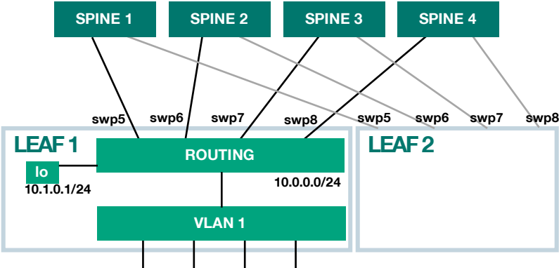
FIGURE 5-4. CREATING A LAYER 3 FABRIC WITH BGP
