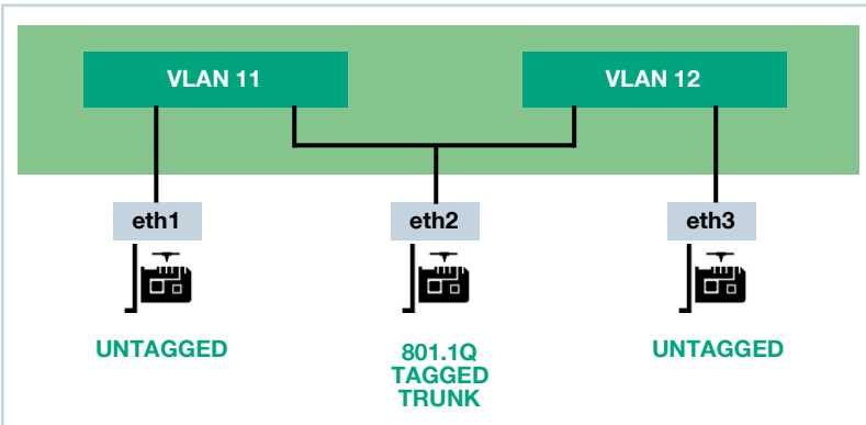
FIGURE 4-3. TAGGED AND UNTAGGED VLAN TRAFFIC
